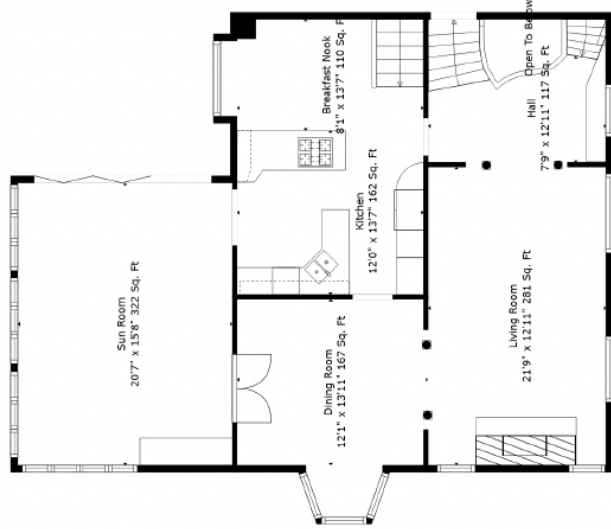
Floor 4
